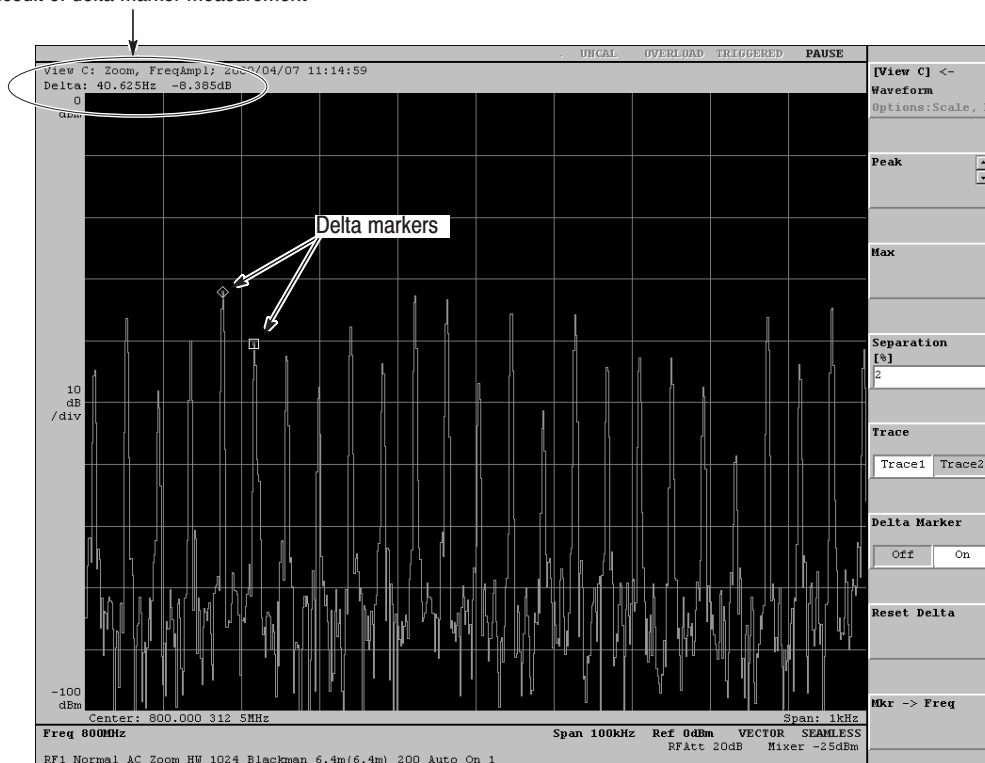
Figure 2-44: Measurement example using the delta markers
