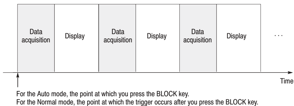
Figure 3-32: Acquiring and displaying data in the Auto and Normal modes
