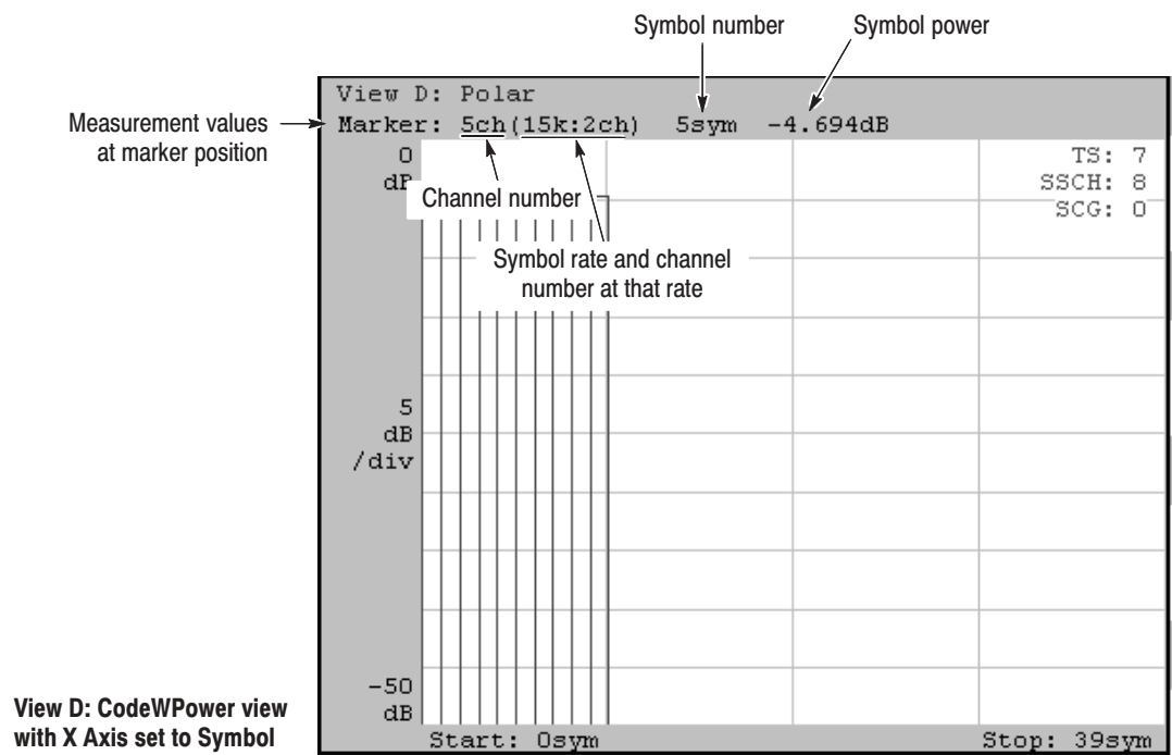
Figure 3-79: Symbol power
