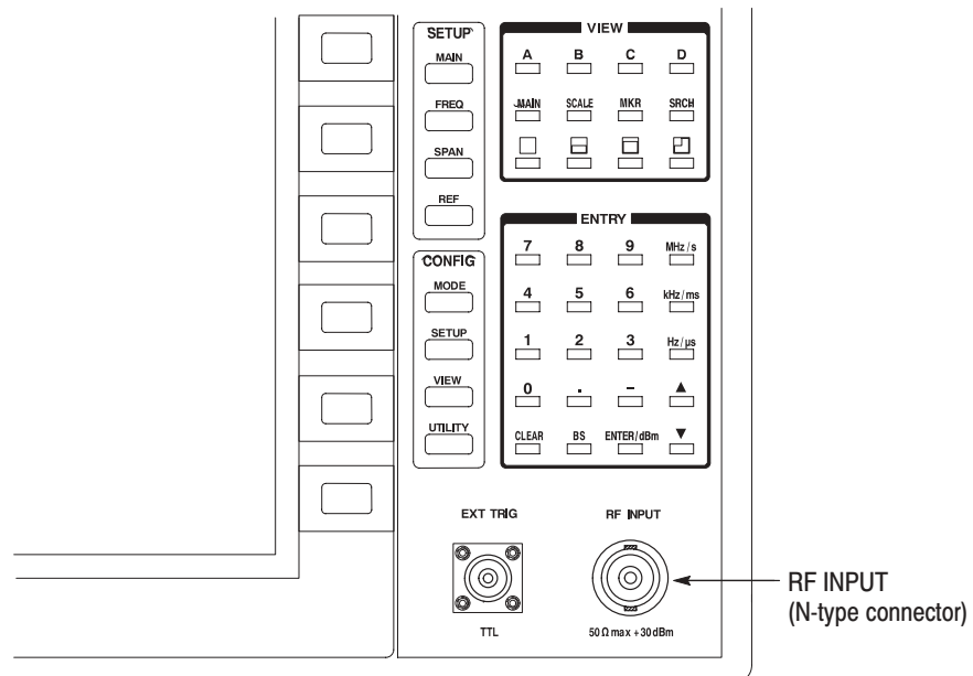
Figure 2–19: Cable connection
