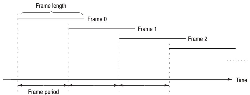
Figure 3–11: Frame period
