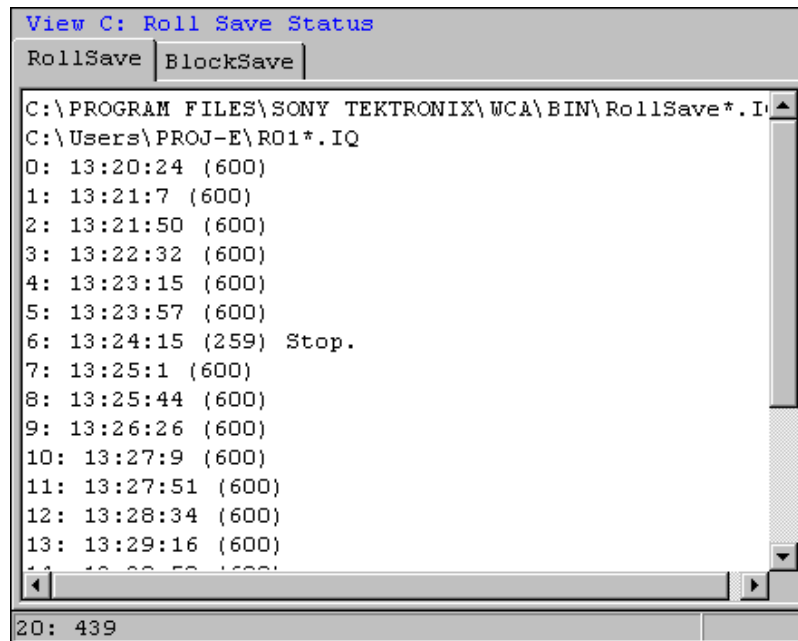
Figure 3-92: Automatic data storage in the Roll mode
