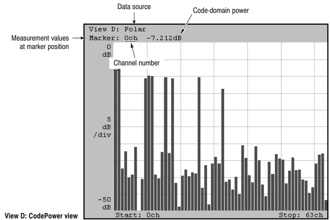
Figure 3-69: Code-domain power
